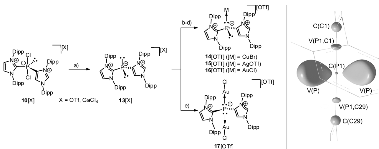
Scheme 4. Reduction of 10 [X] to 13 [X] (left, a) (X = OTf, GaCl 4 ) + 2 K + C 8 H 18 , −2 KCl, THF, −78 °C, 3 h, RT, 14 h; 68 % for 13 [OTf], 85 % for 13 [GaCl 4 ]), reaction of 13 [OTf] with CuBr(tht), Ag[OTf], or AuCl(tht), respectively (middle, b) + CuBr(tht), −0.5 tht, THF, RT, 6 h, 85 % 14 [OTf]; c) + Ag[OTf], THF, −78 °C, 3 h, 78 % 15 [OTf]; d) + AuCl(tht), −tht, THF, RT, 14 h, 92 % 16 [OTf]; [24] e) + 2 AuCl(tht), −tht, THF, RT, 6 h, 88 % 17 [OTf]), and visualization of the ELF at the central [C-P-C] moiety in 13 + (right, 0.948 isosurface). tht = tetrahydrothiophene.
